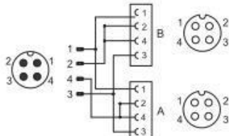
M12 Y3型连接器电路图
