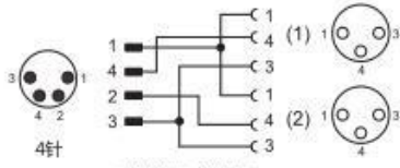
M8-Y2型连接器电路图
