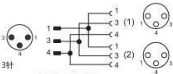
M8-Y1型连接器电路图
