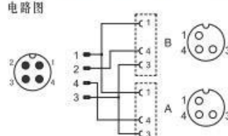
M12 Y2型连接器电路图
